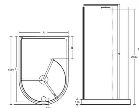
Serenis 360 peninsular walk in enclosure - right hand tray illustrated
