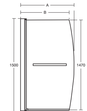
Bow bath screen with towel rail
