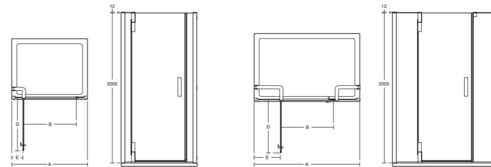
Tonic alcove 800mm - 1000mm left hand version illustrated
