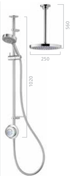
Length of hose: 1500. Ceiling arm can be cut to suit site conditions.
