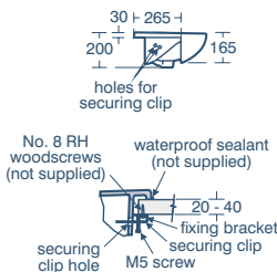
section through basin showing securing clip
