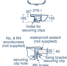
section through basin showing securing clip
