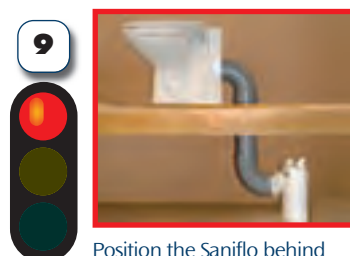
Position the Saniflo behind the toilet not underneath it.
