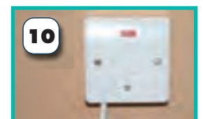
Electrical connection should be via an unswitched fixed wiring connector with a 5 amp fuse.
