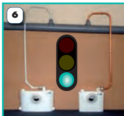
Each Saniflo discharge pipe should run separately to the soil pipe. If wastes are combined, it can only be into a larger pipe, which is on a gravity fall.
