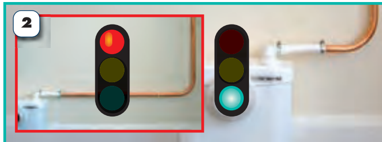
Bends should be smooth/long radius, not tight elbows. (Examples of copper and plastic shown).
