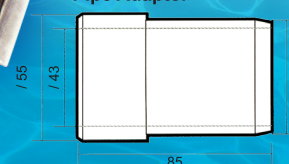
Pipe Adaptor
