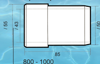
Pipe Adaptor
