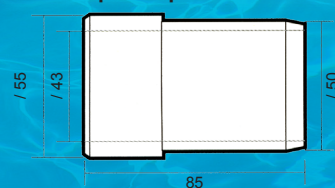
Pipe Adaptor
